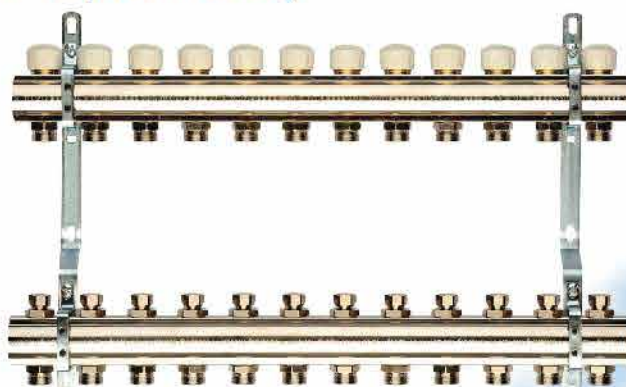
6500.93: Distribution manifold with mechanical balancing screw 1" (from T4 to T7) 1" 1/4 (from T4 to T12)
